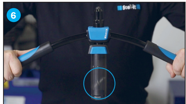
6 After breaking the mandrel, hold the tool vertically and spread the arms to release mandrel into the collector.
